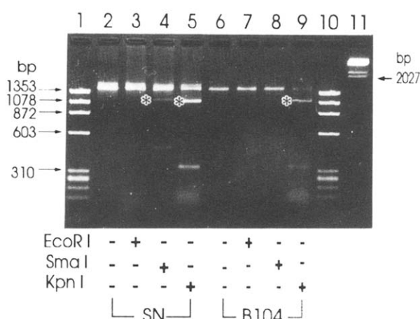
Fig. 3. RT-PCR amplification of the rat brain Na + channel \alpha subunit using primer set B. Restriction mapping analysis (run on 2% agarose gel) in sciatic nerve (SN; lanes 2–5) and B104 cells (B104; lanes 6–9). Lanes 1 and 10 contain \phi X174/ Hae III digests, and lane 11 contains lambda DNA/ Hind III fragments. Lanes 2 and 6 are the amplified PCR products without restriction enzyme treatment. PCR products were treated with subtype specific enzymes in the amplified regions: Eco R I (subtype I-specific, lanes 3,7); Sma I (subtype II-specific, lanes 4,8); or Kpn I (subtype III-specific, lanes 5,9). The asterisks indicate the largest enzyme-digested fragment for the respective subtypes. The results demonstrate the presence of subtype II and III mRNAs in sciatic nerve and only subtype III mRNA in B104 cells.
